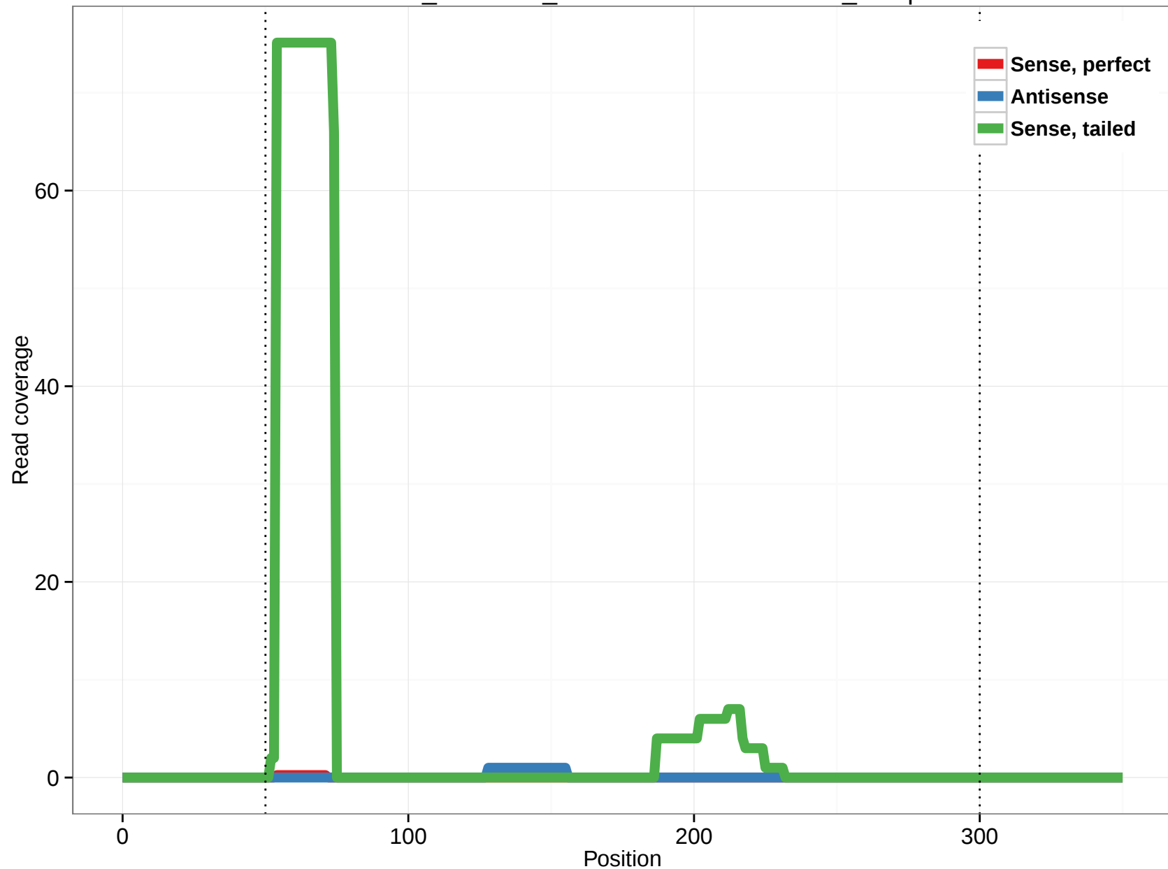
ornAna1_ensGene_ENSOANT00000021130_12.5p
