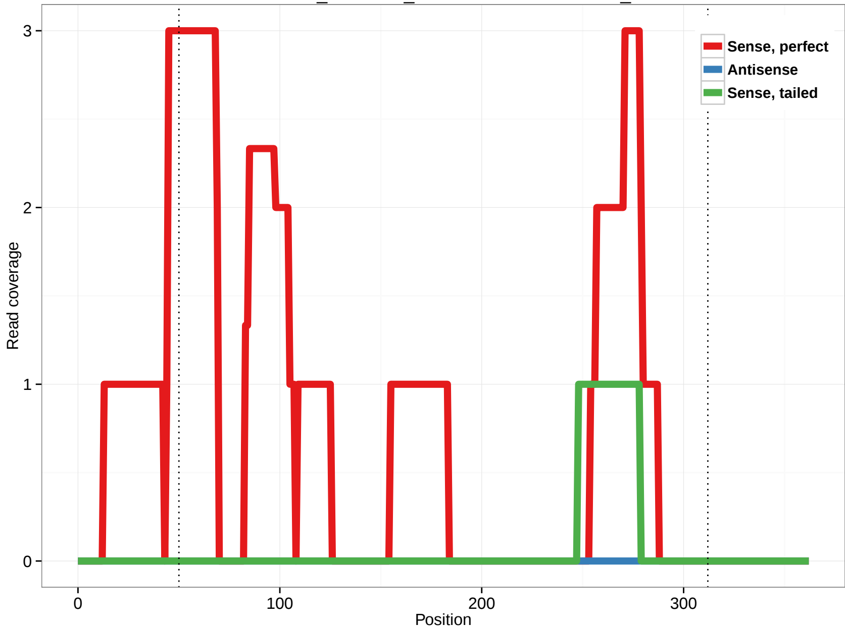
ornAna1_ensGene_ENSOANT00000021127_1
