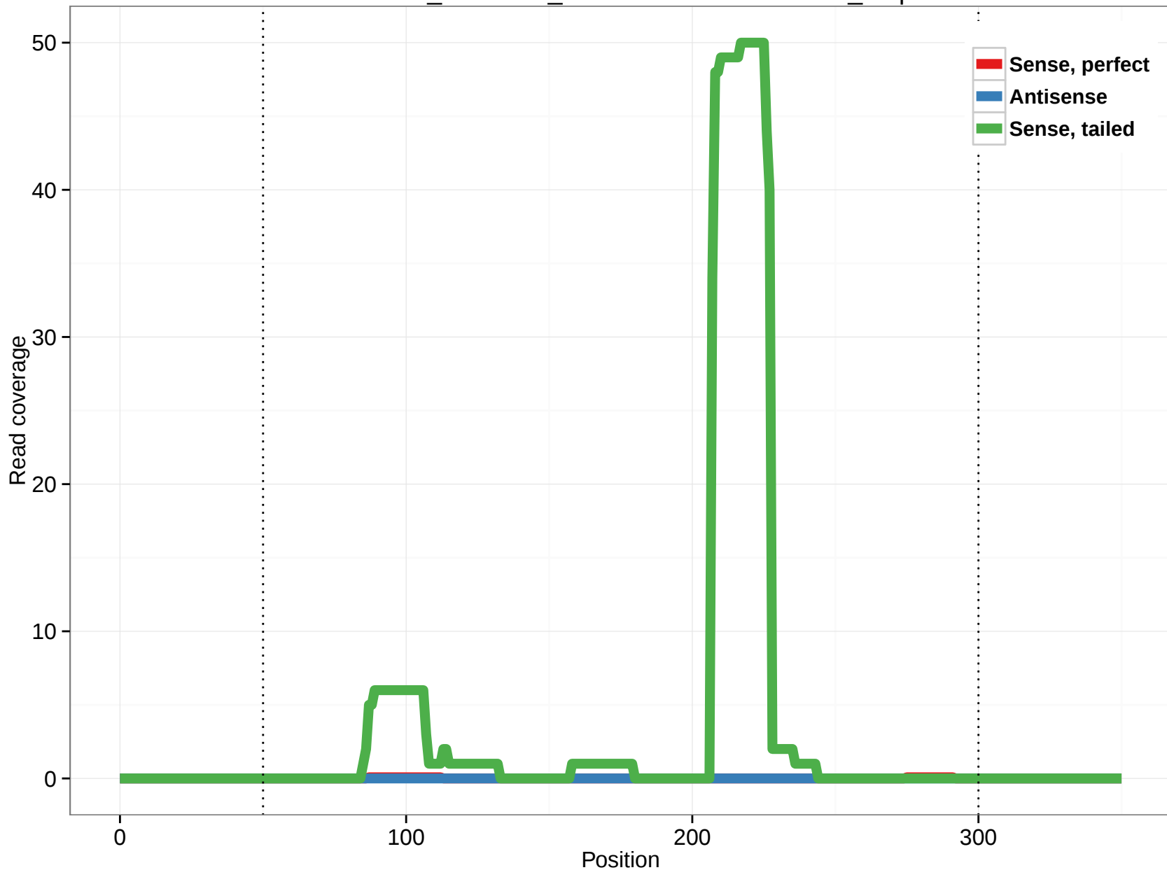
ornAna1_ensGene_ENSOANT00000021119_5.3p
