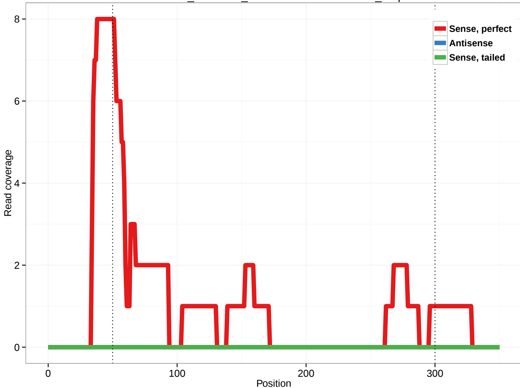
ornAna1_ensGene_ENSOANT00000021107_6.5p
