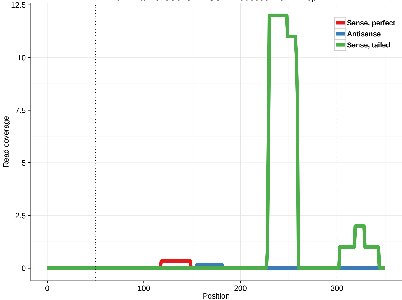
ornAna1_ensGene_ENSOANT00000021044_2.5p
