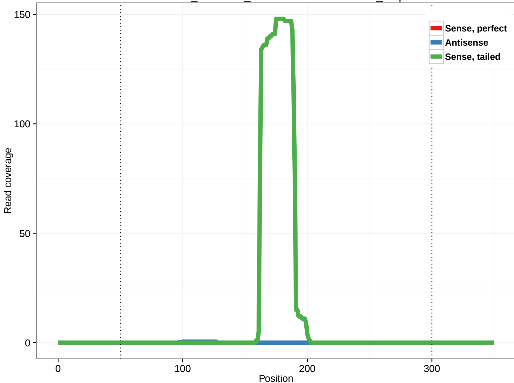
ornAna1_ensGene_ENSOANT00000021041_7.3p
