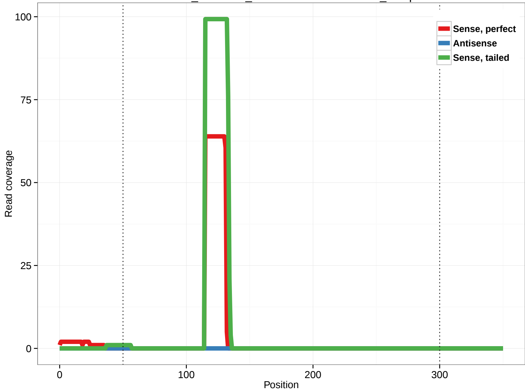
ornAna1_ensGene_ENSOANT00000021036_10.5p
