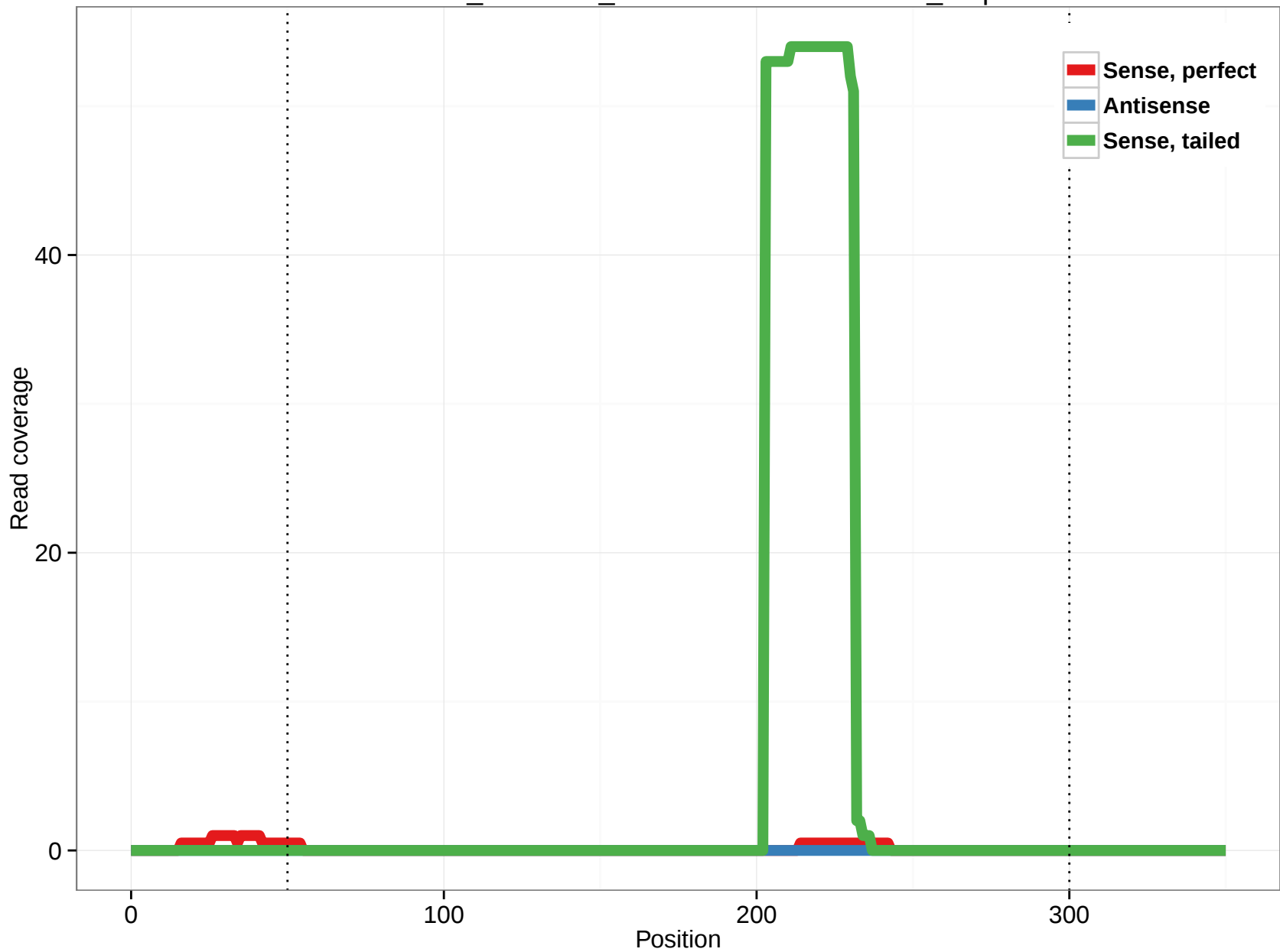
ornAna1_ensGene_ENSOANT00000021036_1.5p
