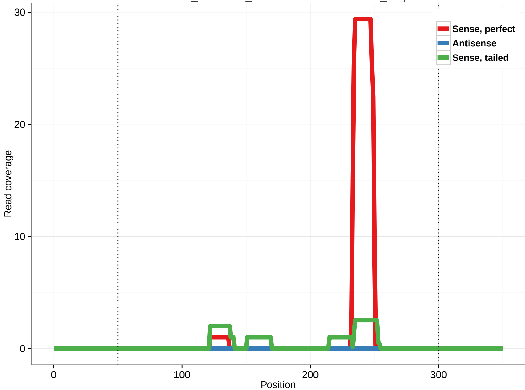
ornAna1_ensGene_ENSOANT00000020969_3.3p
