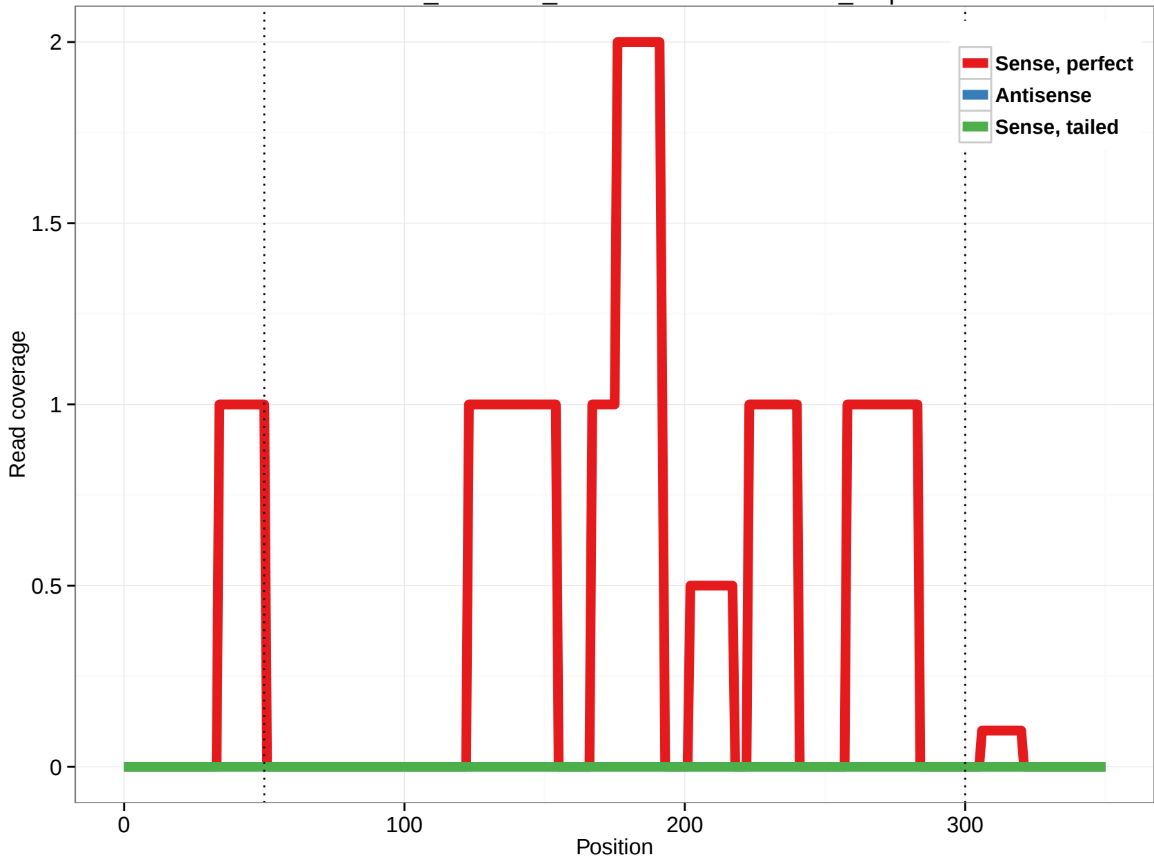
ornAna1_ensGene_ENSOANT00000020939_1.5p
