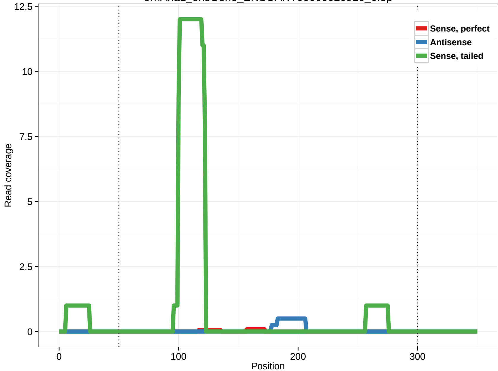
ornAna1_ensGene_ENSOANT00000020910_0.5p
