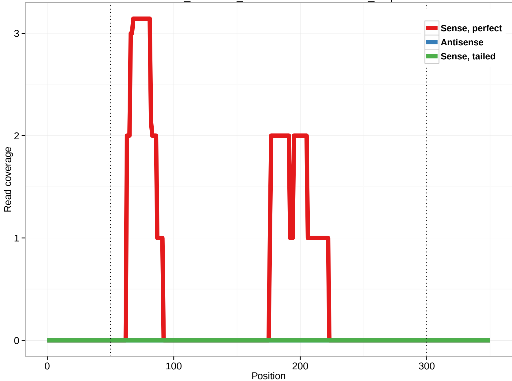
ornAna1_ensGene_ENSOANT00000020868_0.3p
