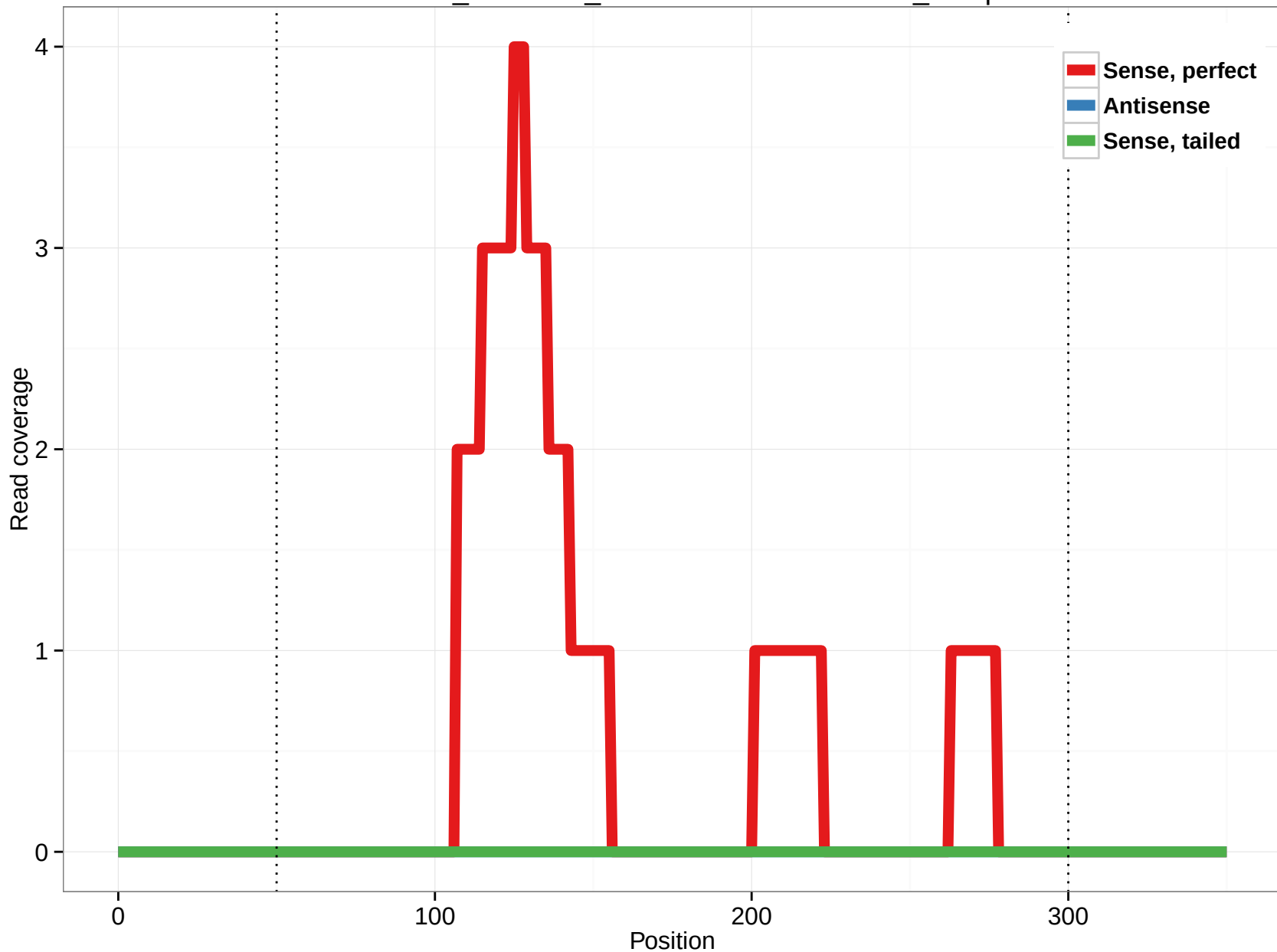
ornAna1_ensGene_ENSOANT00000020863_17.3p
