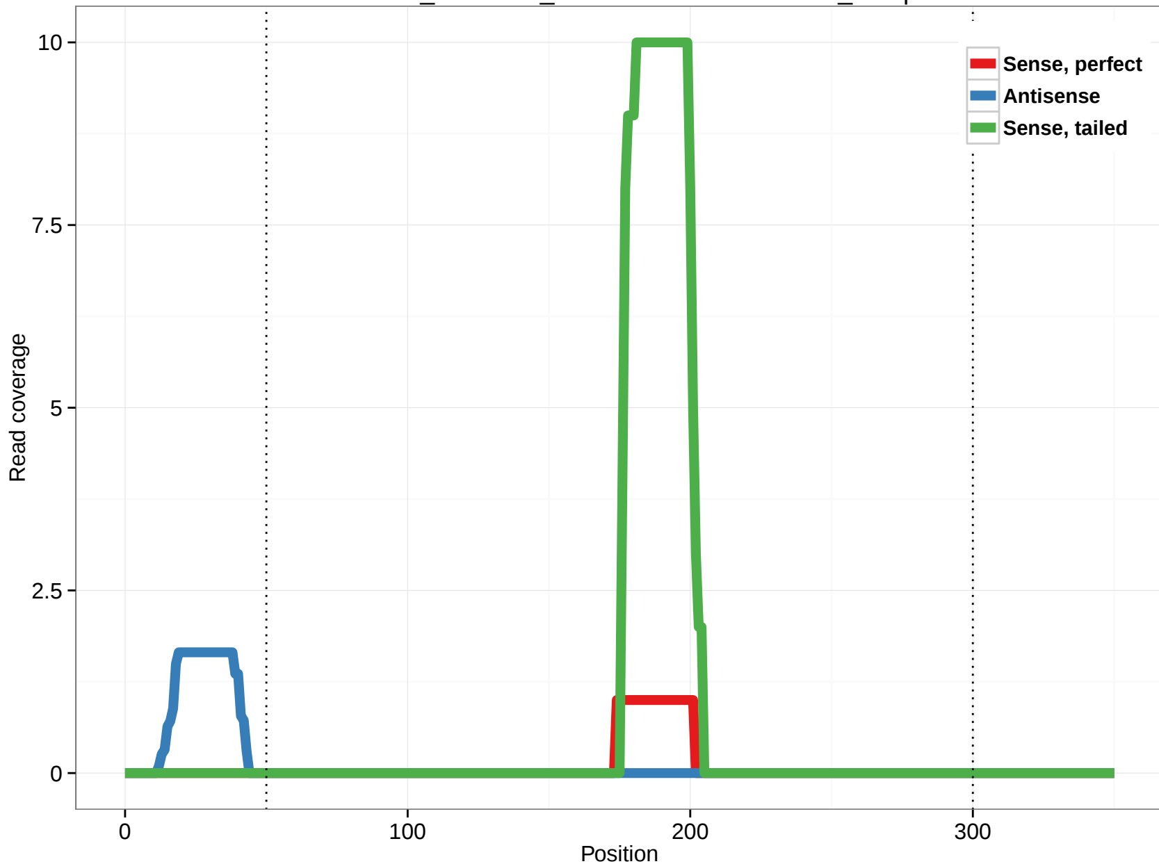
ornAna1_ensGene_ENSOANT00000020757_11.3p
