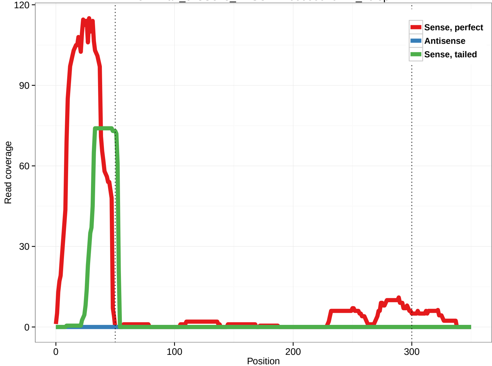
ornAna1_ensGene_ENSOANT00000020724_10.5p
