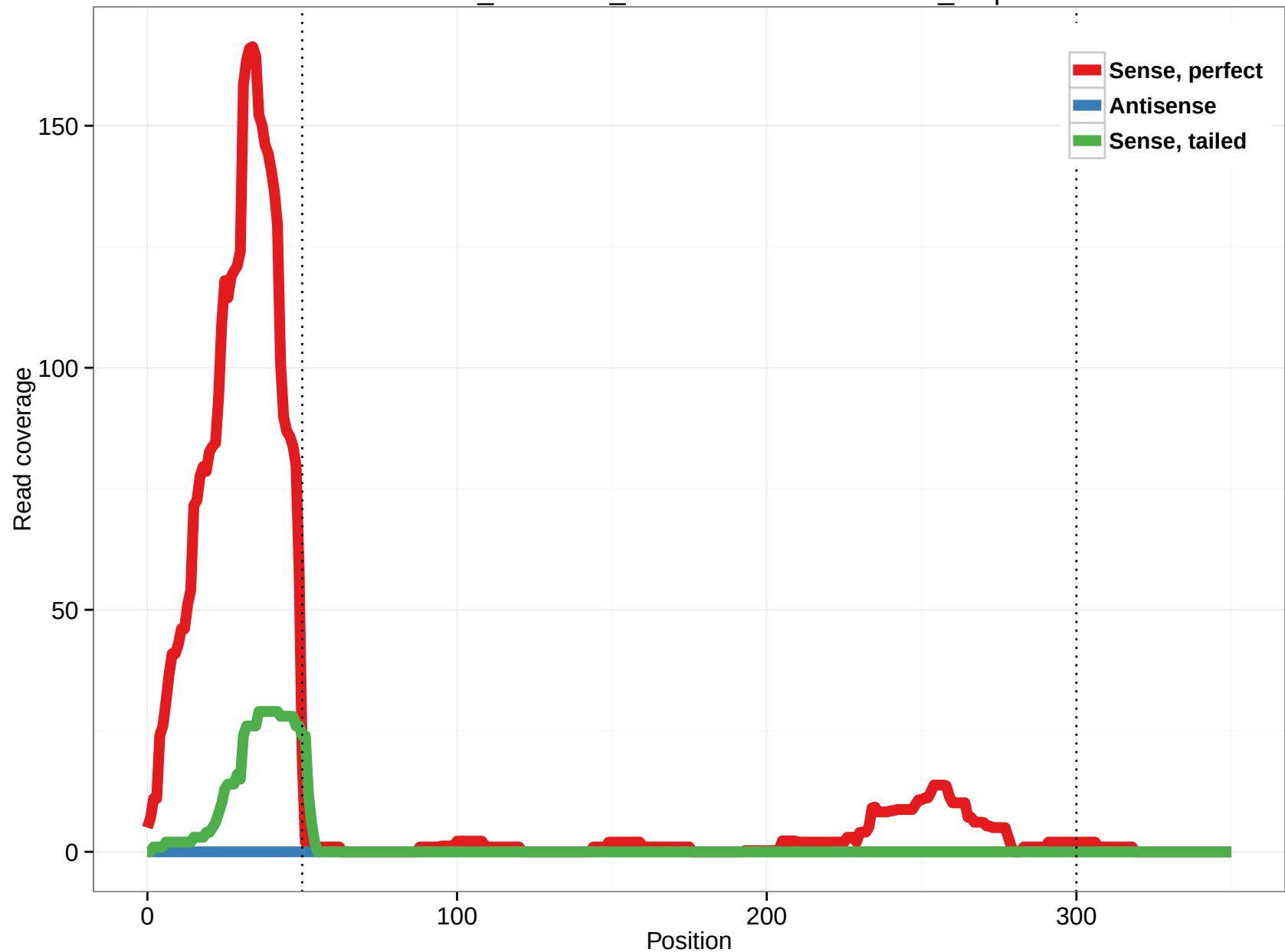
ornAna1_ensGene_ENSOANT00000020724_0.5p
