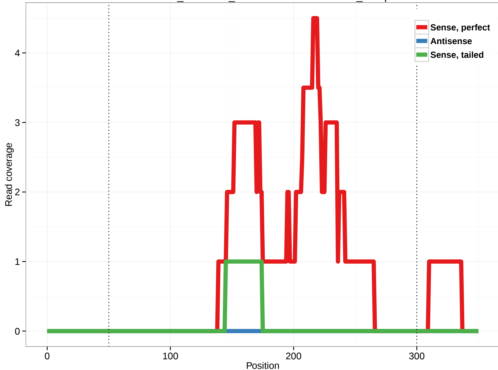
ornAna1_ensGene_ENSOANT00000020644_14.3p
