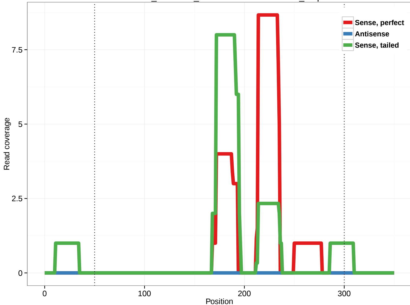
ornAna1_ensGene_ENSOANT00000020569_7.5p
