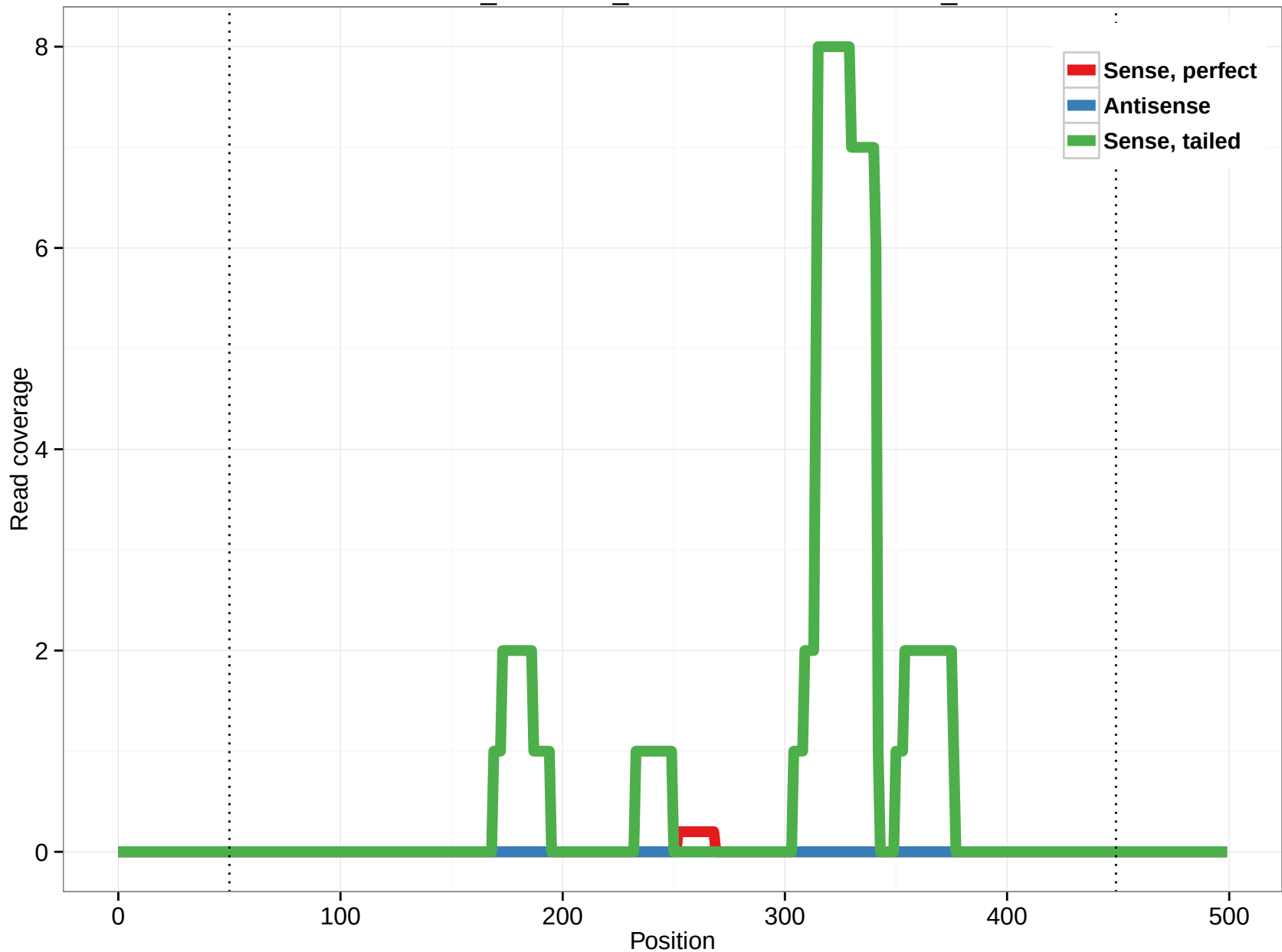
ornAna1_ensGene_ENSOANT00000020561_0
