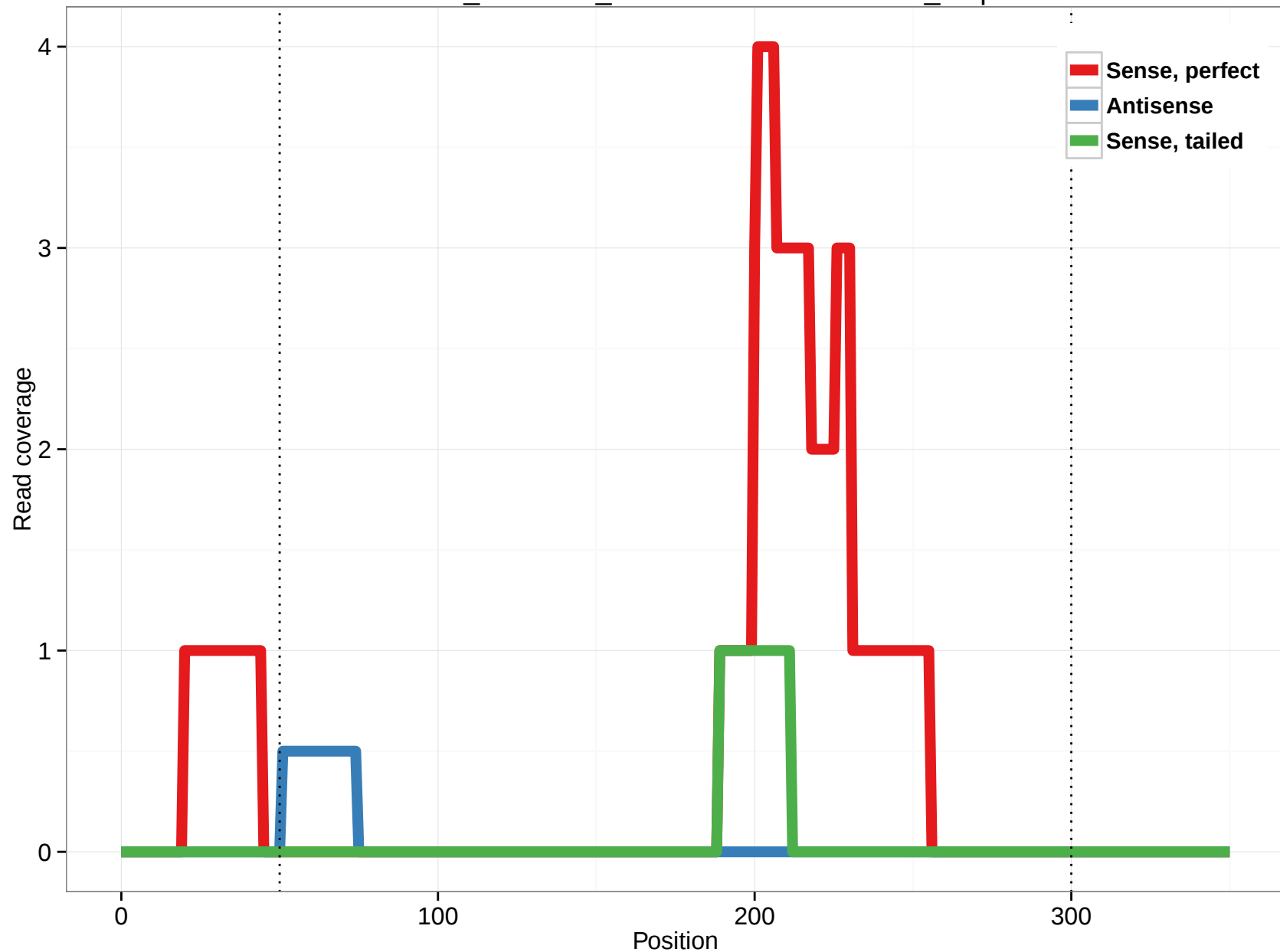
ornAna1_ensGene_ENSOANT00000020457_1.3p
