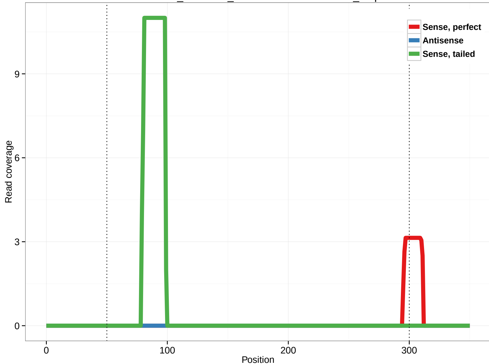
ornAna1_ensGene_ENSOANT00000020390_0.3p
