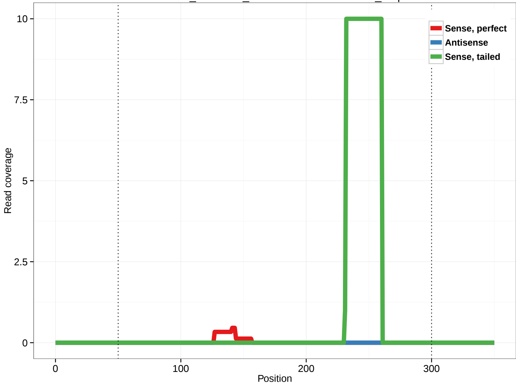
ornAna1_ensGene_ENSOANT00000020386_2.3p
