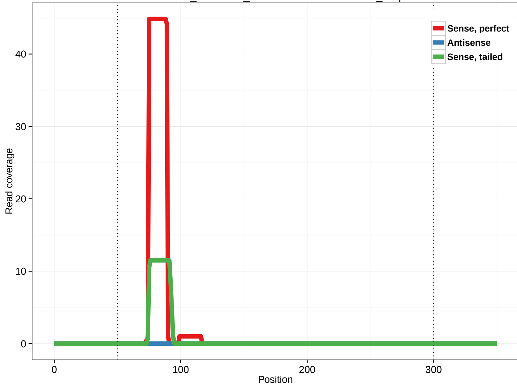
ornAna1_ensGene_ENSOANT00000020364_7.3p
