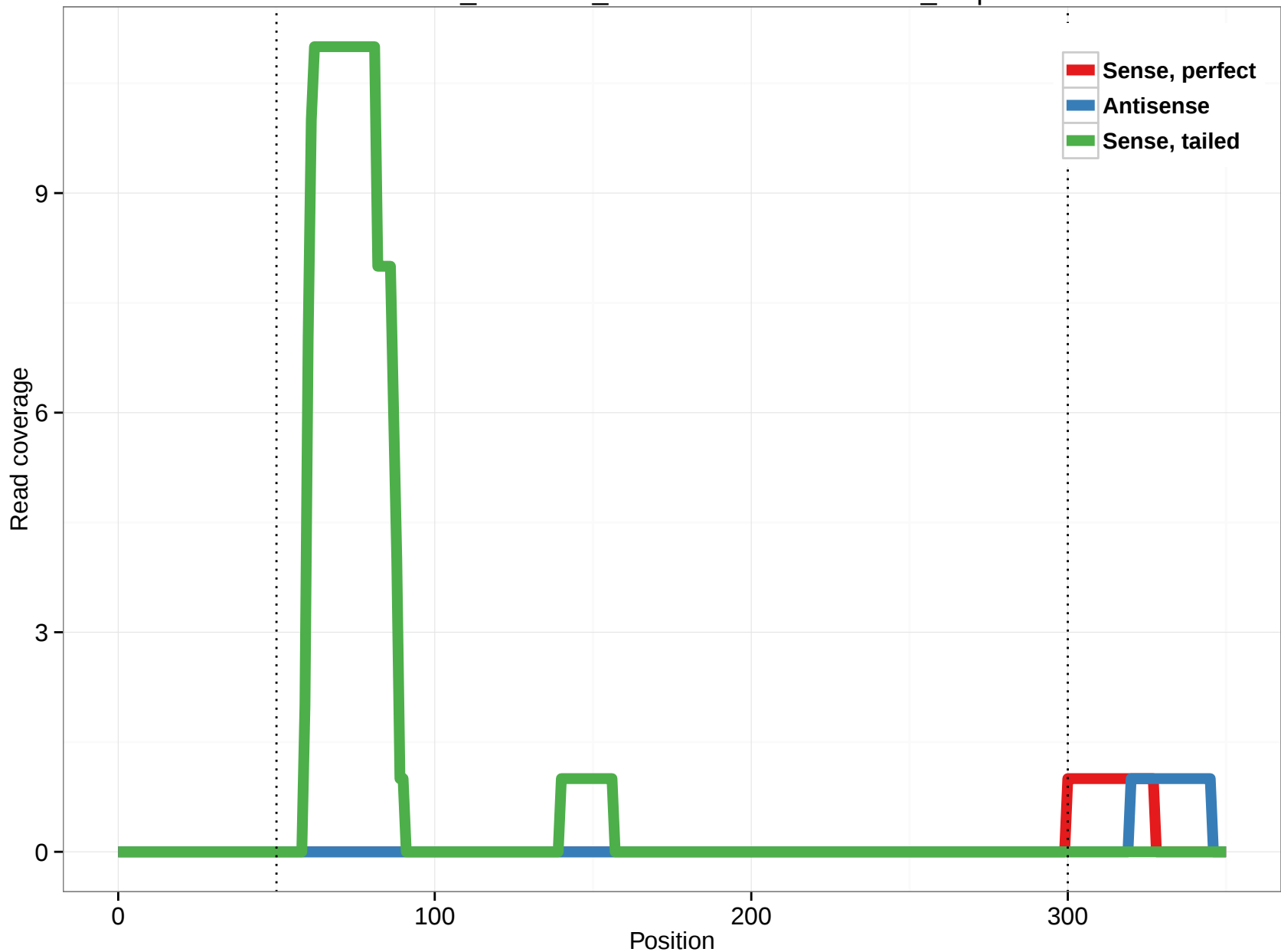
ornAna1_ensGene_ENSOANT00000020363_4.3p
