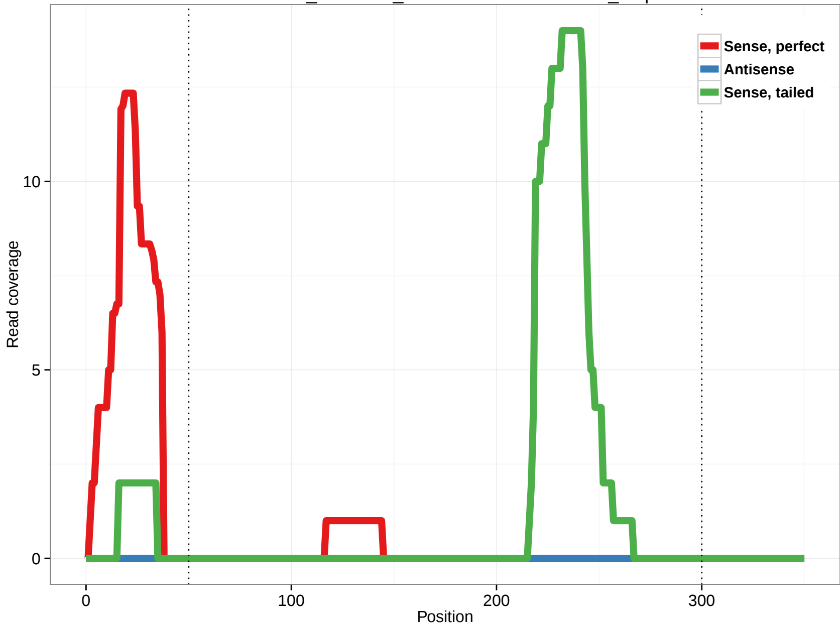
ornAna1_ensGene_ENSOANT00000020273_2.5p
