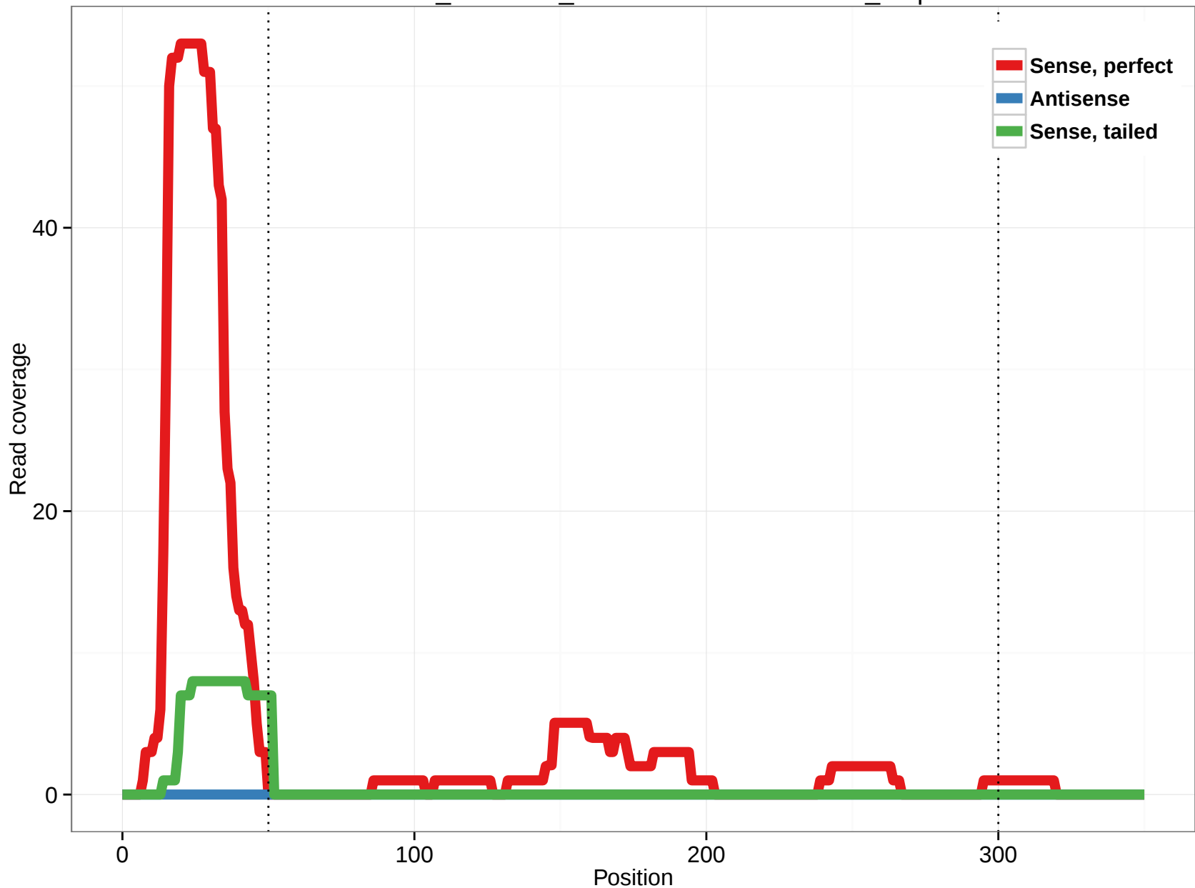
ornAna1_ensGene_ENSOANT00000020224_2.5p
