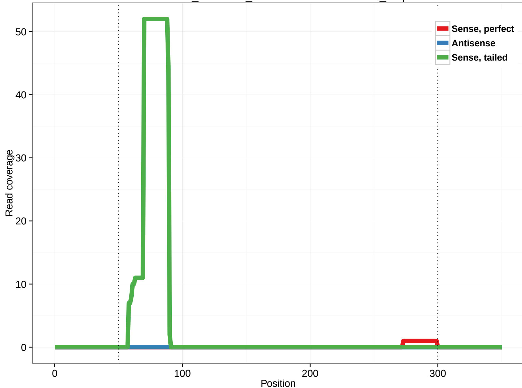
ornAna1_ensGene_ENSOANT00000020046_3.3p
