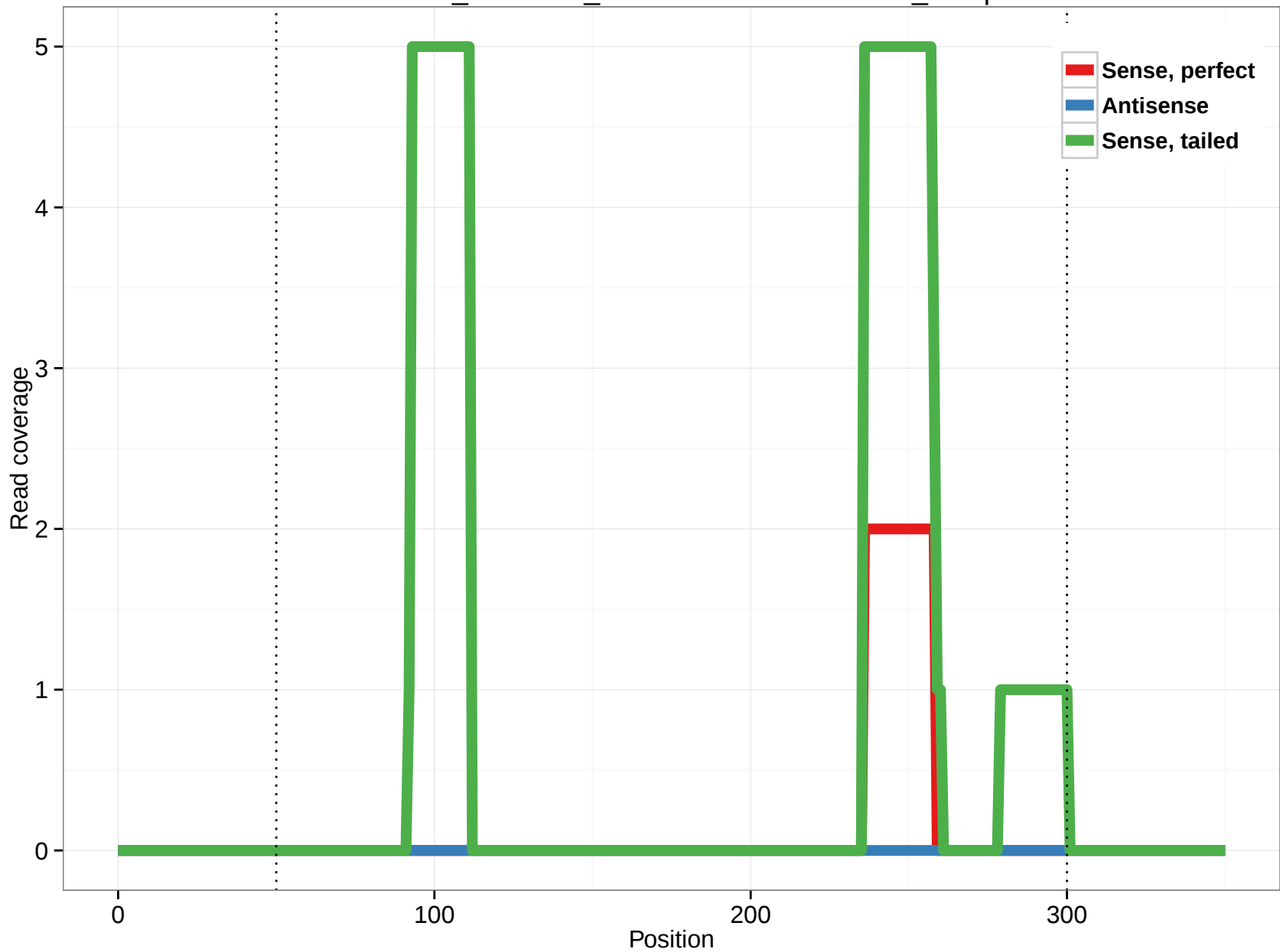
ornAna1_ensGene_ENSOANT00000020046_12.3p
