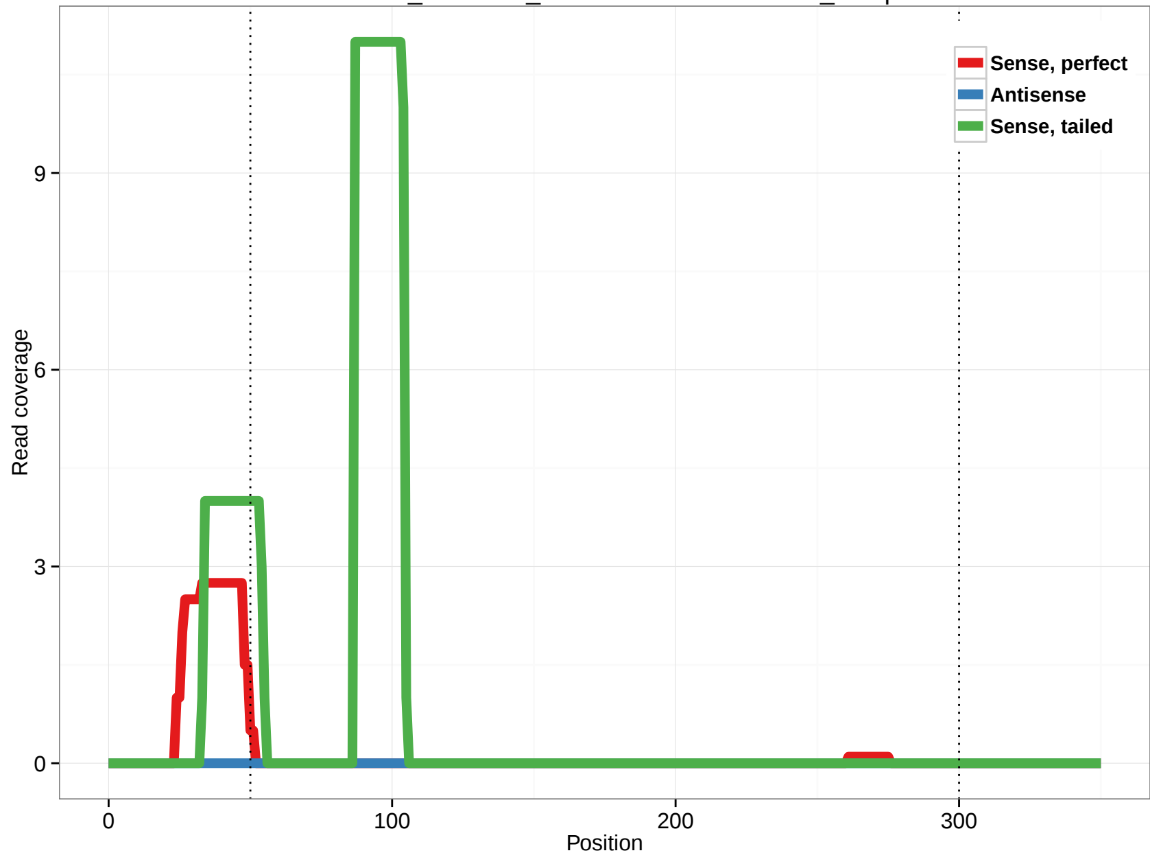
ornAna1_ensGene_ENSOANT00000020036_20.5p
