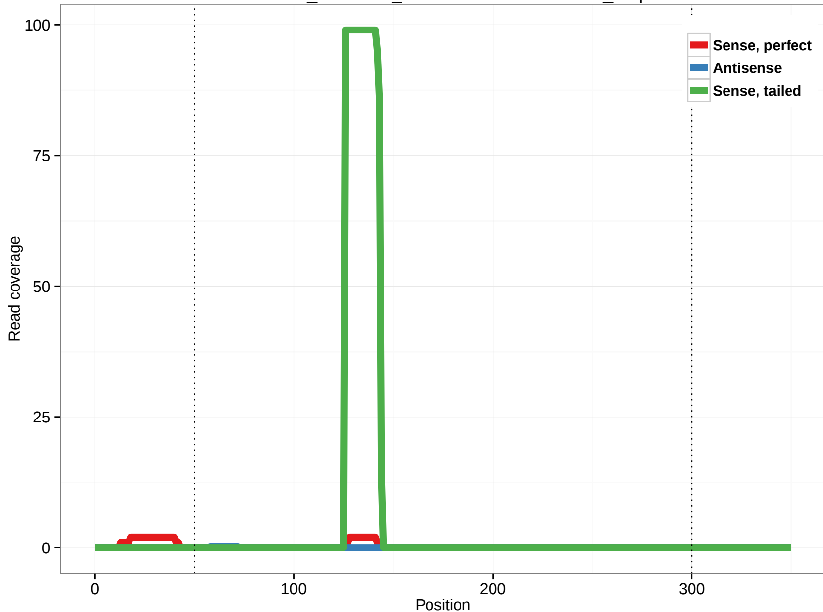
ornAna1_ensGene_ENSOANT00000019900_7.5p
