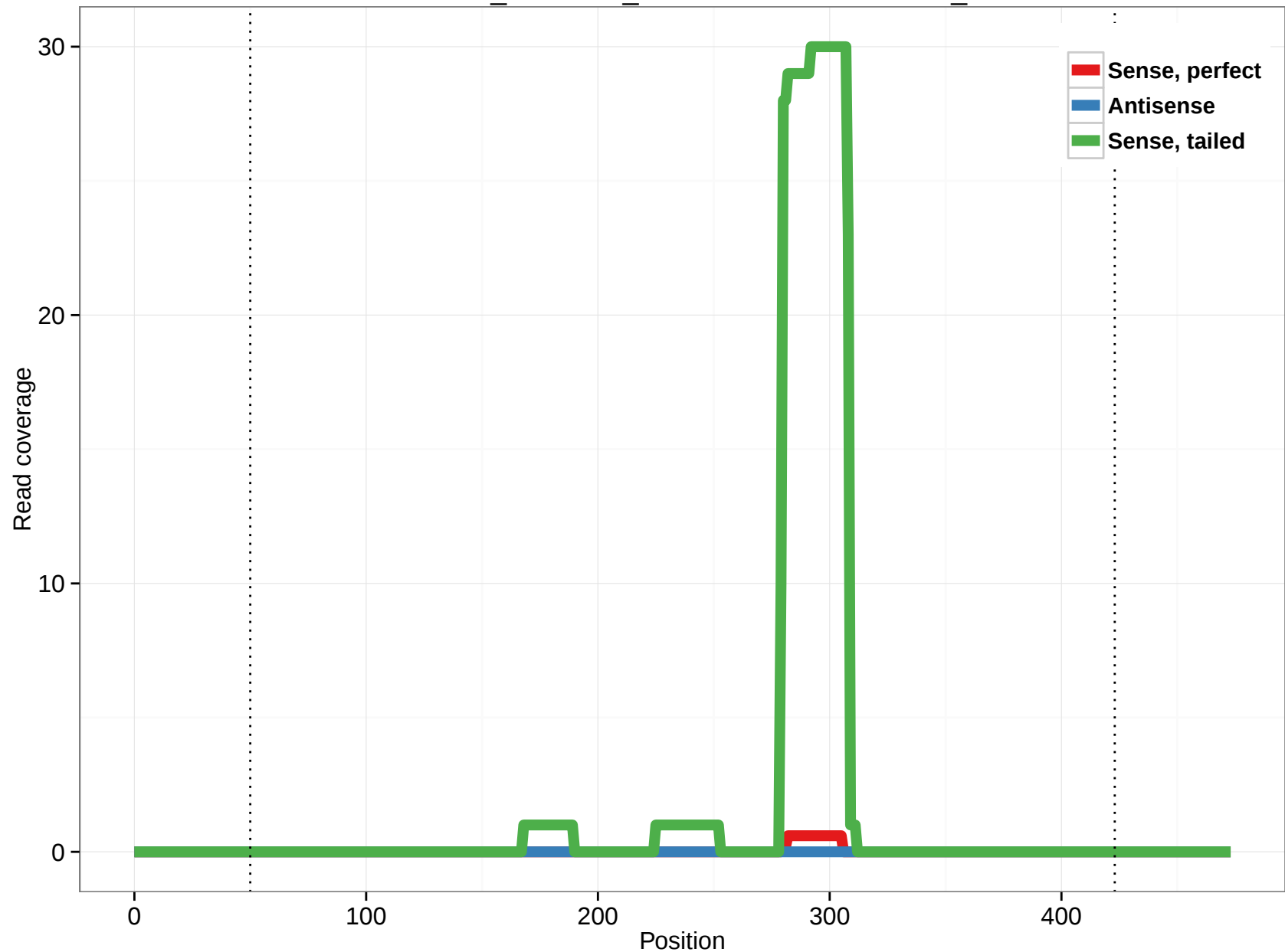
ornAna1_ensGene_ENSOANT00000019892_0
