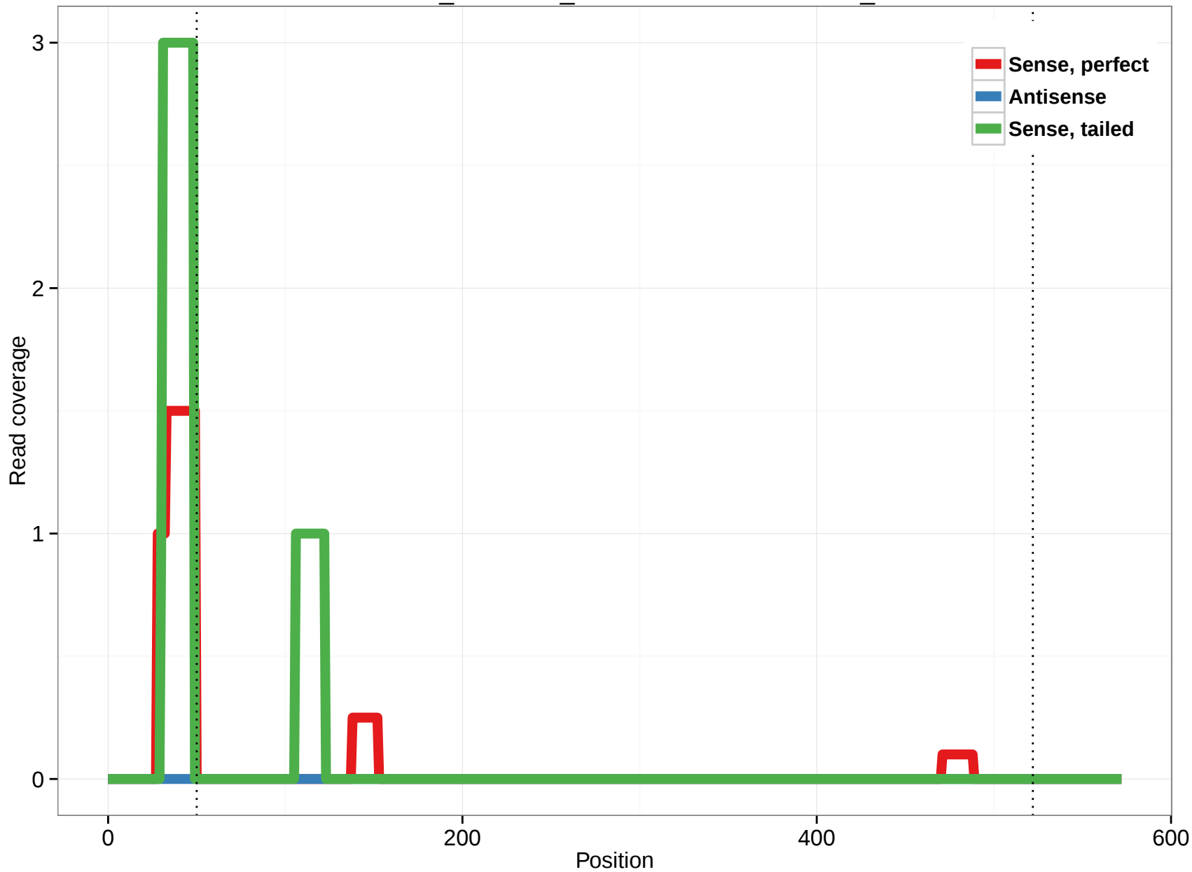
ornAna1_ensGene_ENSOANT00000019862_5
