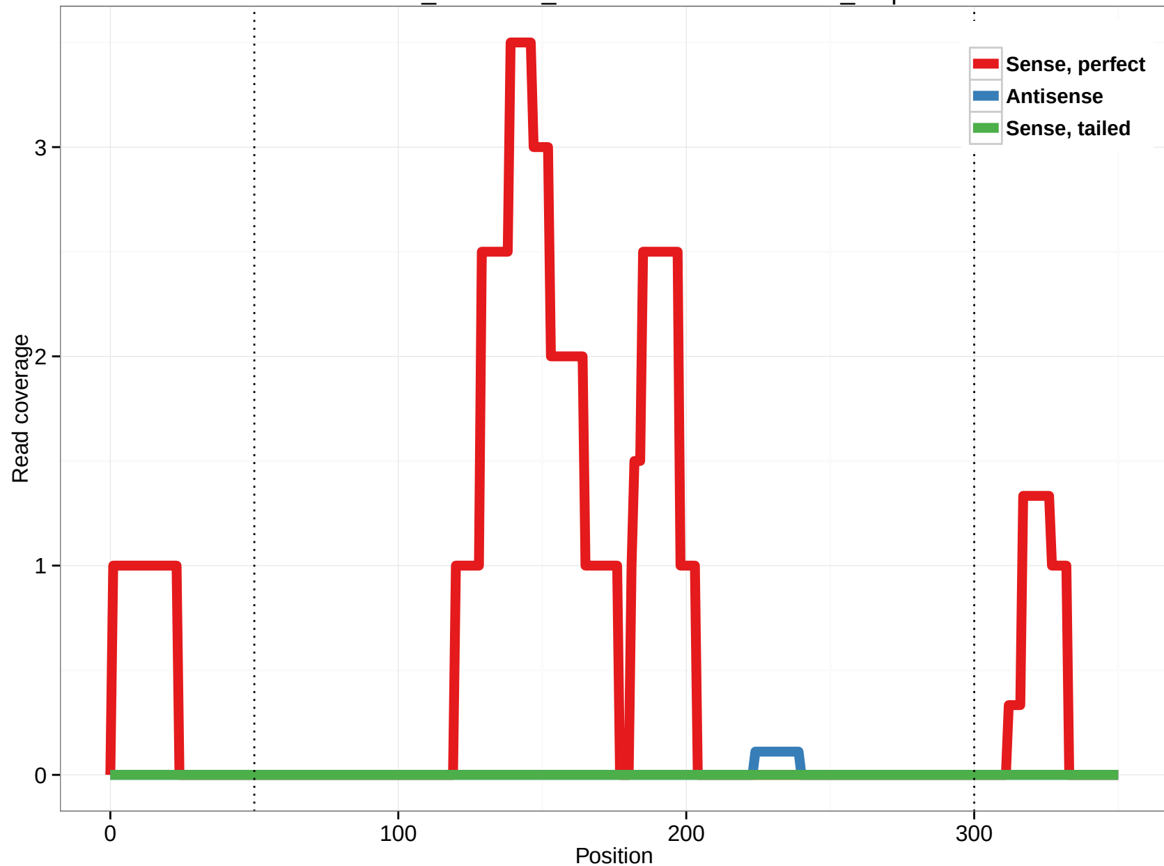
ornAna1_ensGene_ENSOANT00000019724_5.5p
