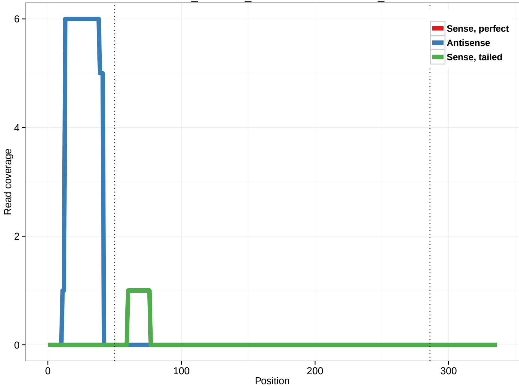
ornAna1_ensGene_ENSOANT00000019708_19
