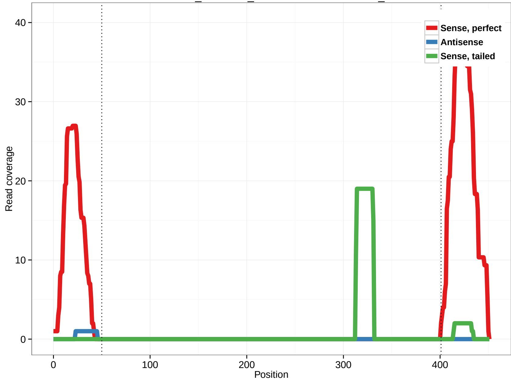
ornAna1_ensGene_ENSOANT00000019699_2
