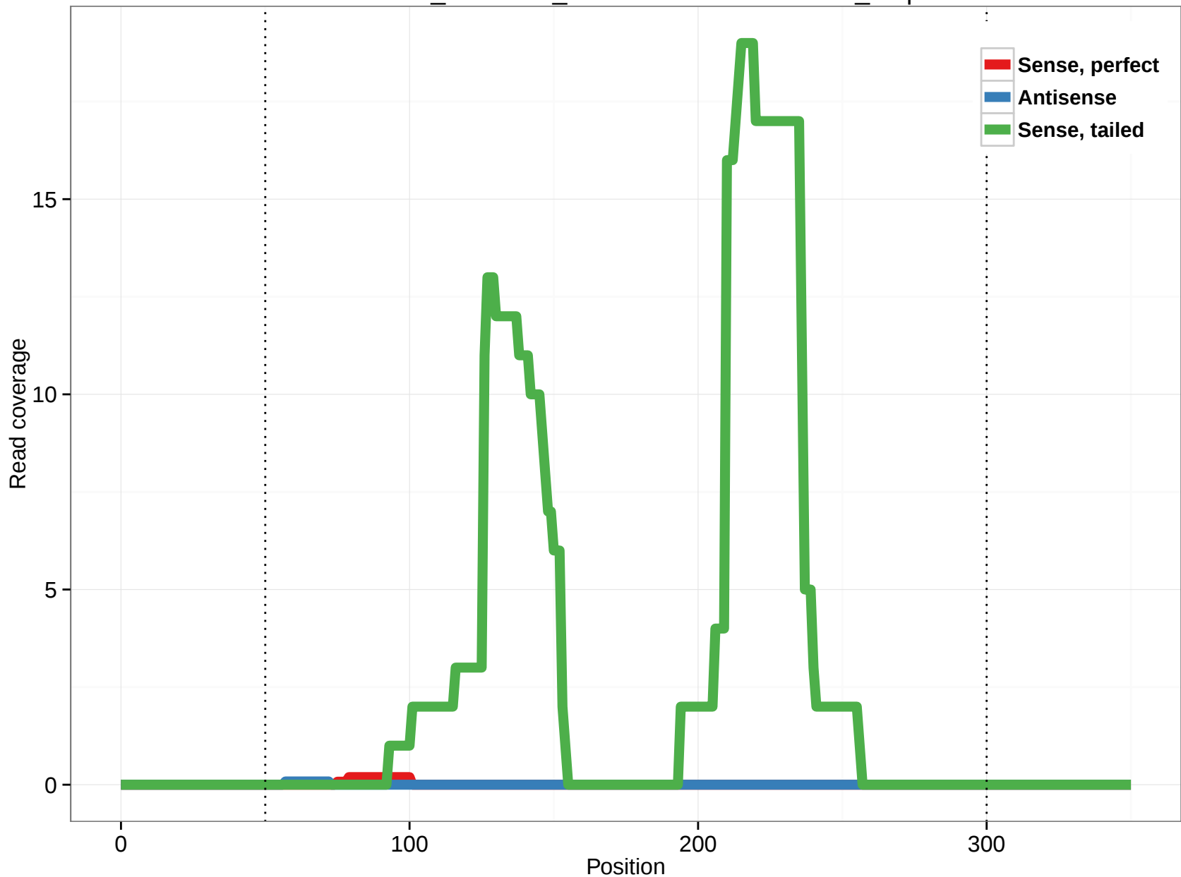
ornAna1_ensGene_ENSOANT00000019636_2.5p
