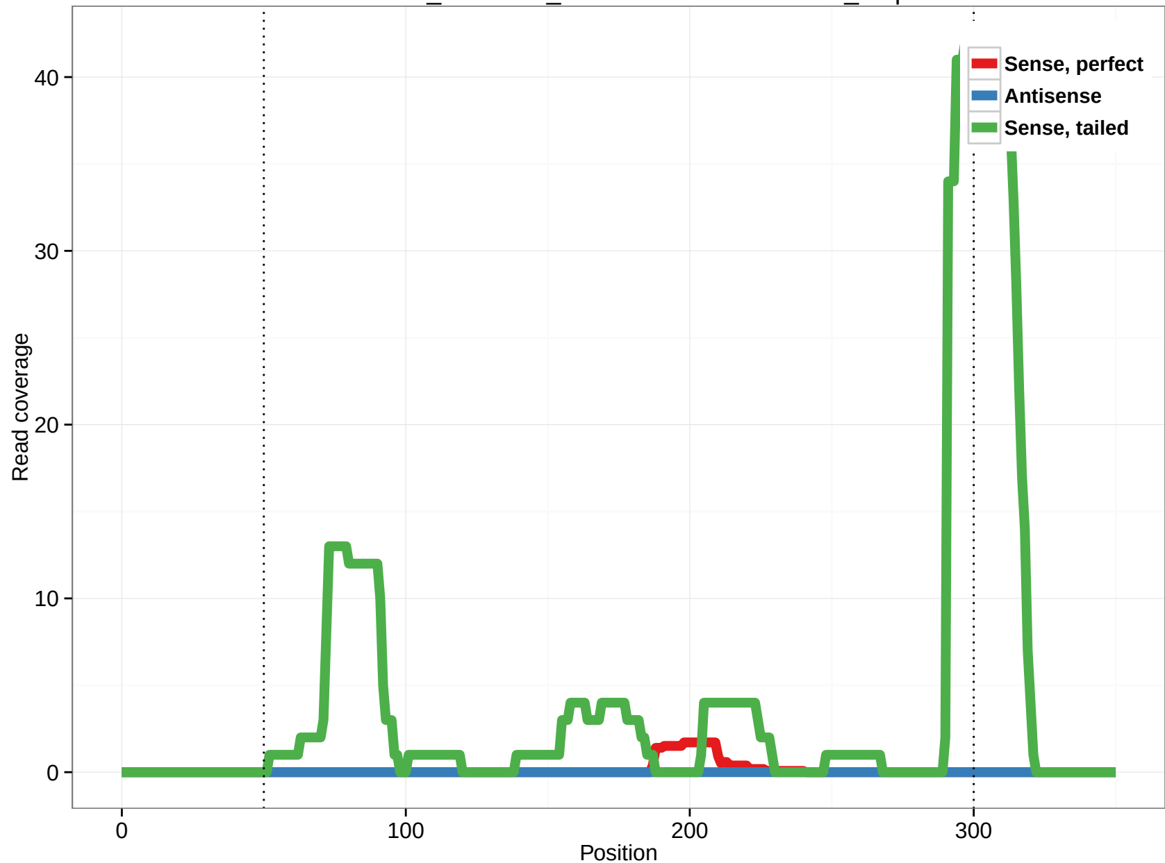
ornAna1_ensGene_ENSOANT00000019636_1.5p
