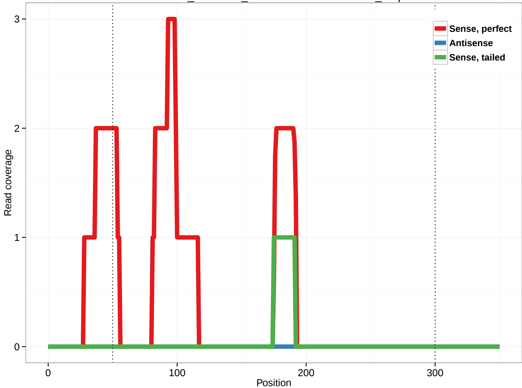
ornAna1_ensGene_ENSOANT00000019622_5.5p
