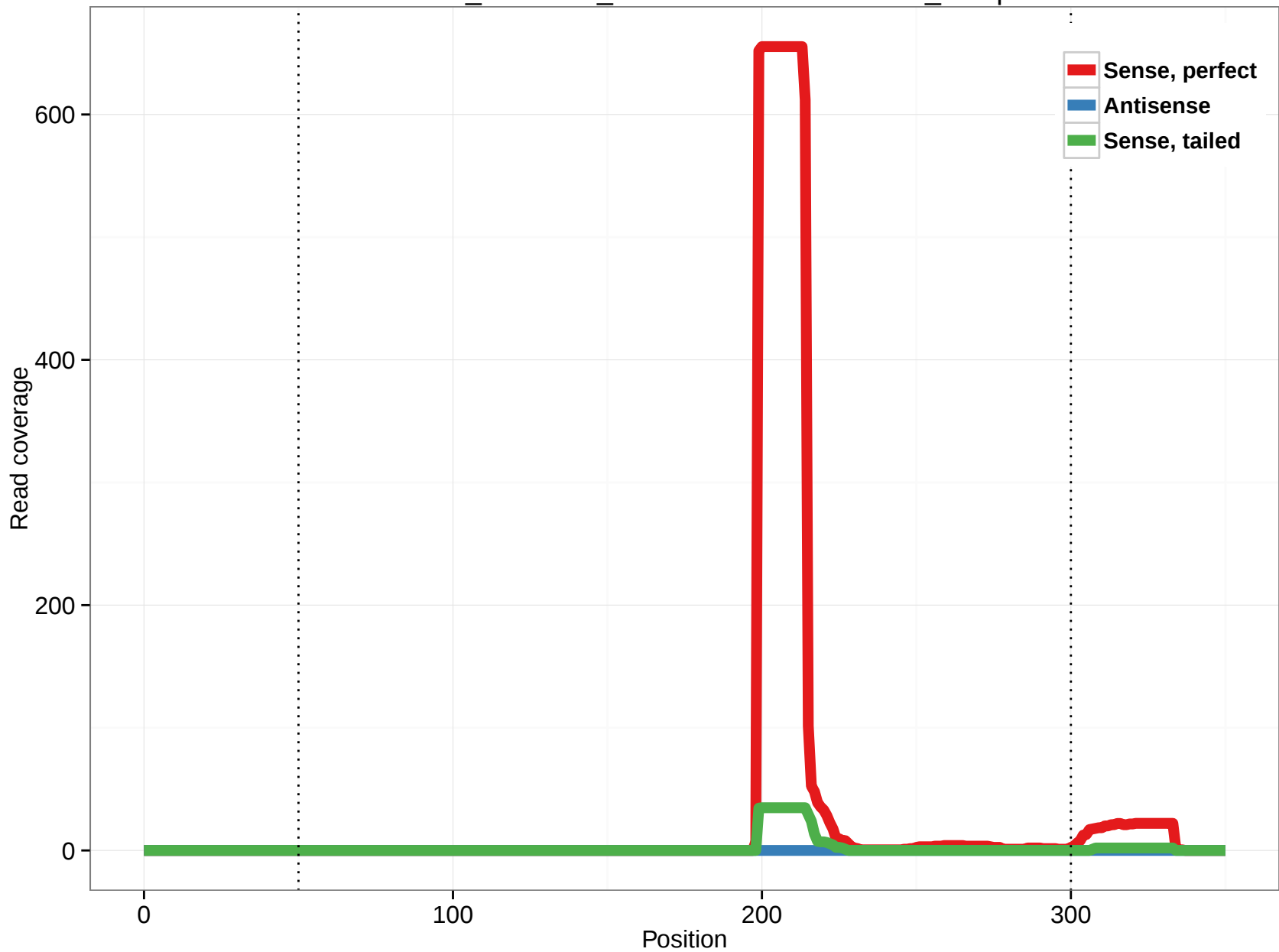
ornAna1_ensGene_ENSOANT00000019597_24.5p
