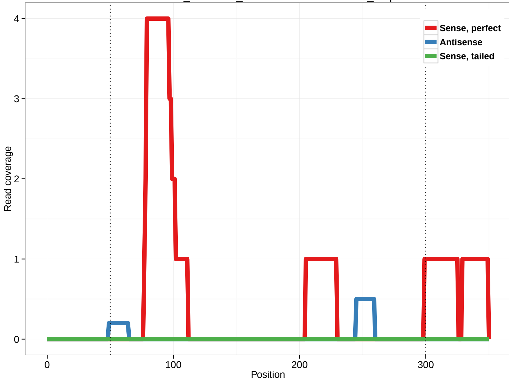
ornAna1_ensGene_ENSOANT00000019573_6.3p
