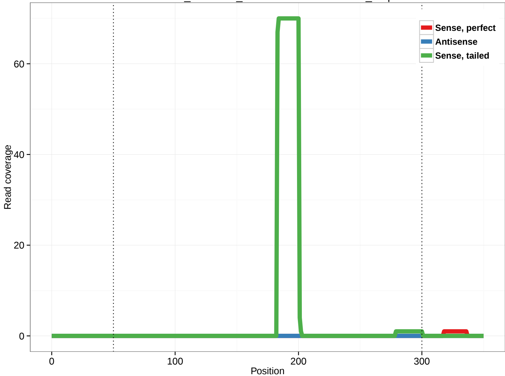
ornAna1_ensGene_ENSOANT00000019550_9.3p
