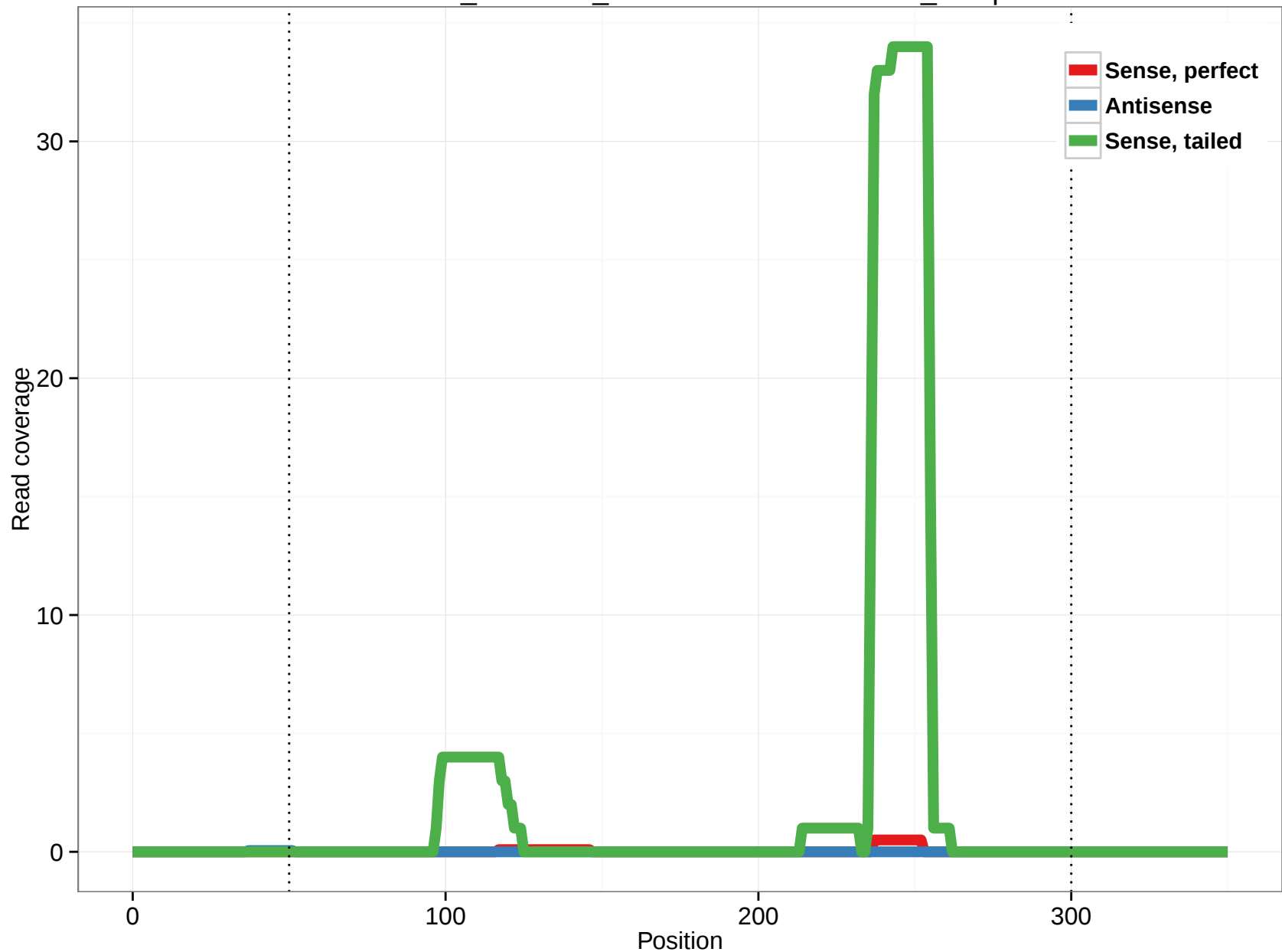
ornAna1_ensGene_ENSOANT00000019507_10.5p
