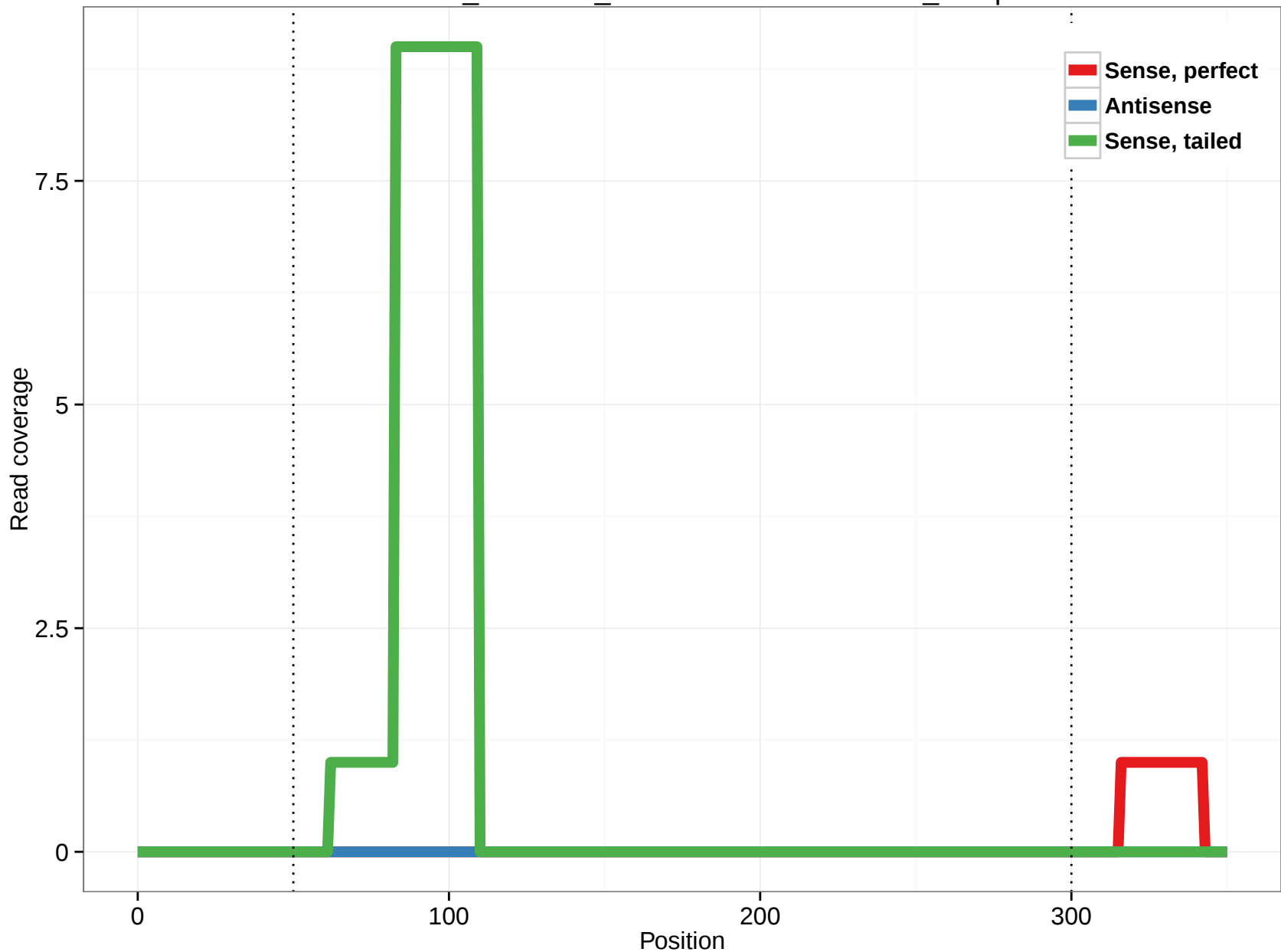
ornAna1_ensGene_ENSOANT00000019396_17.3p
