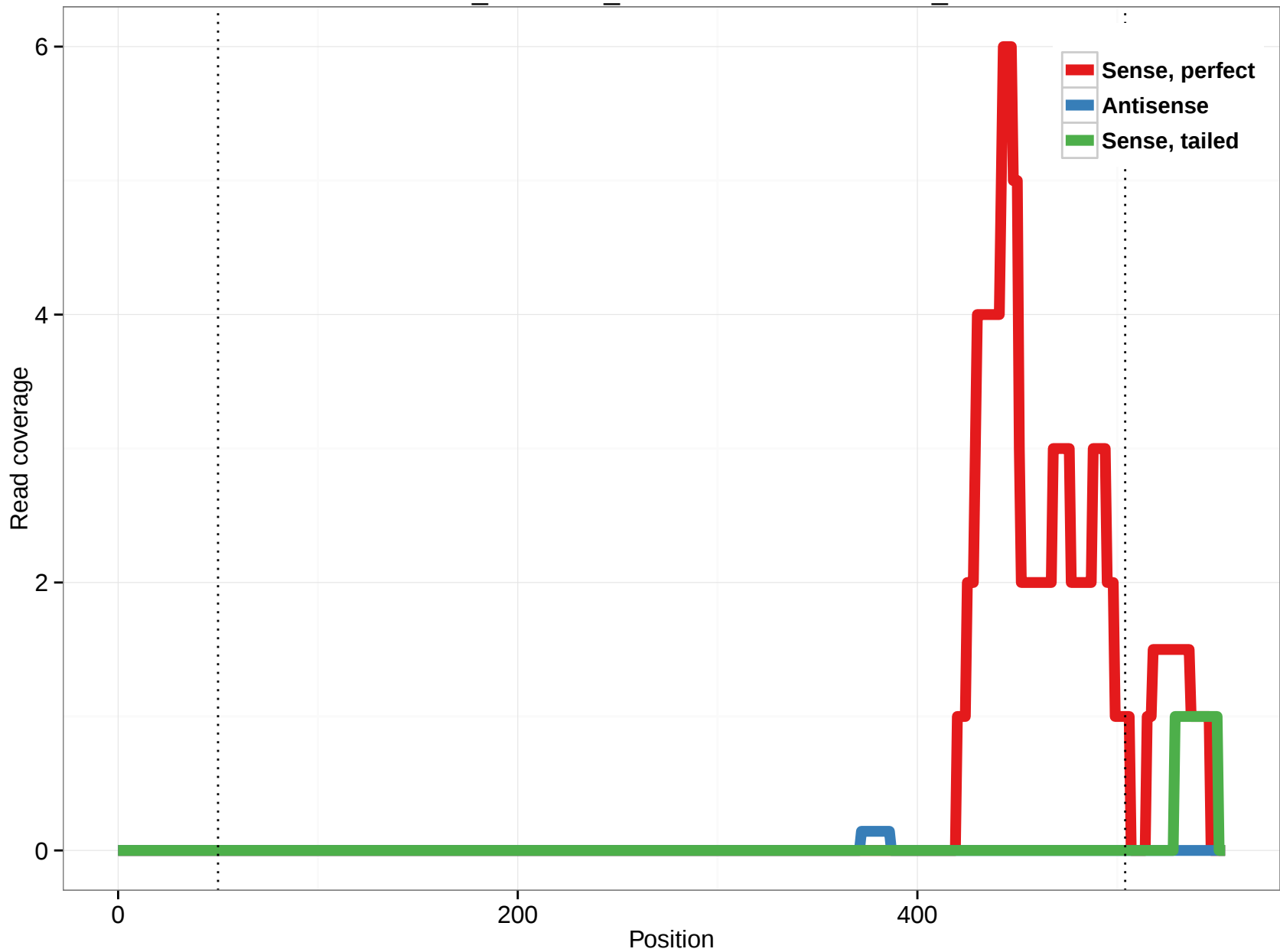
ornAna1_ensGene_ENSOANT00000019366_28
