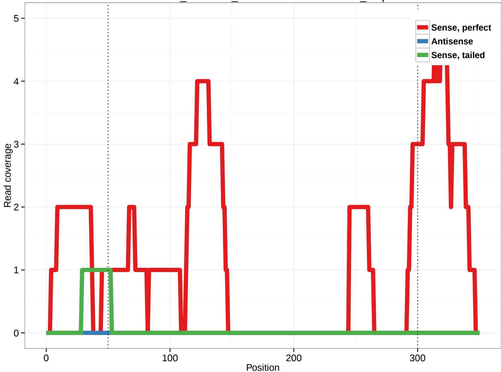
ornAna1_ensGene_ENSOANT00000019356_4.5p
