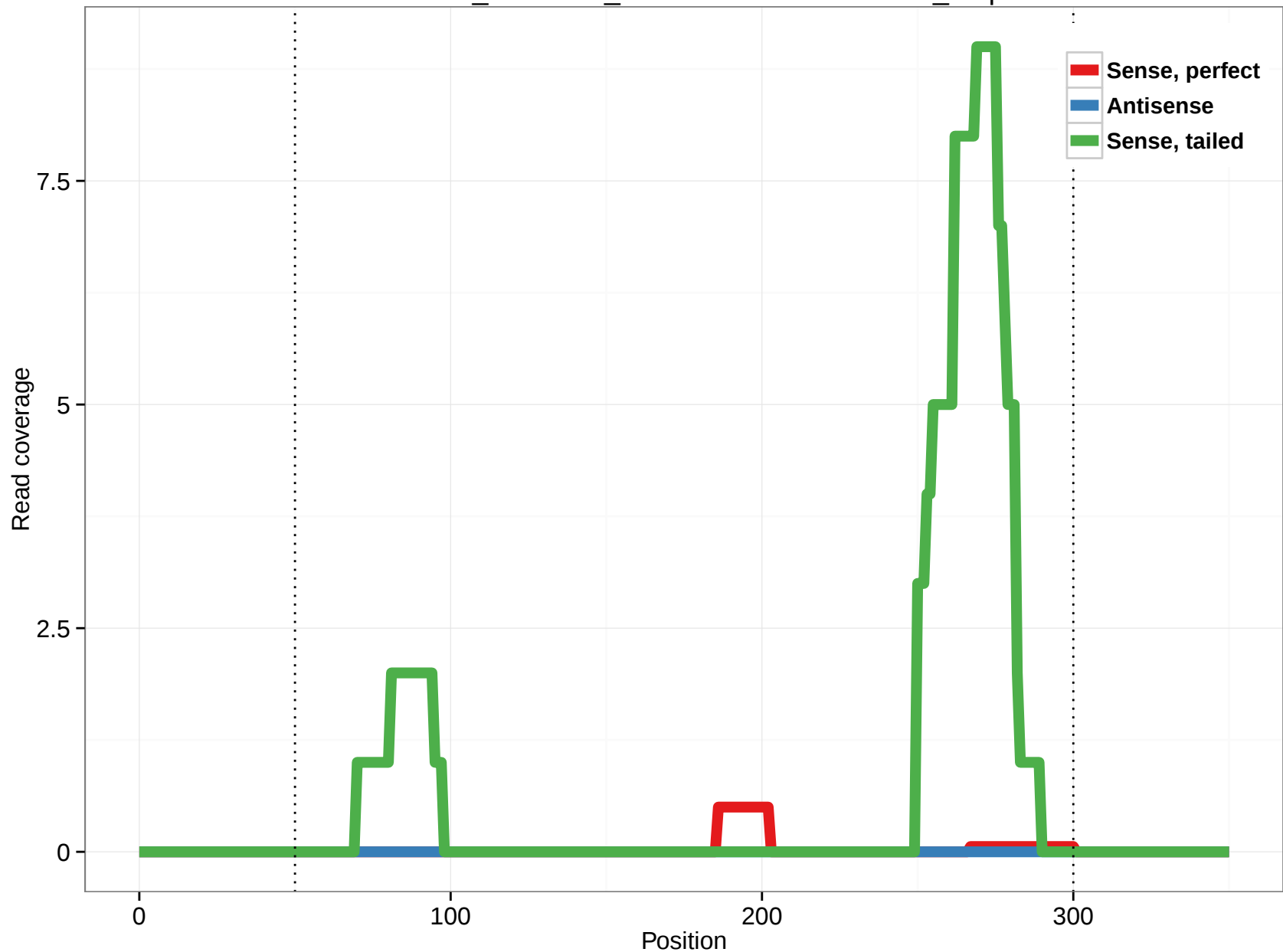
ornAna1_ensGene_ENSOANT00000019347_8.5p
