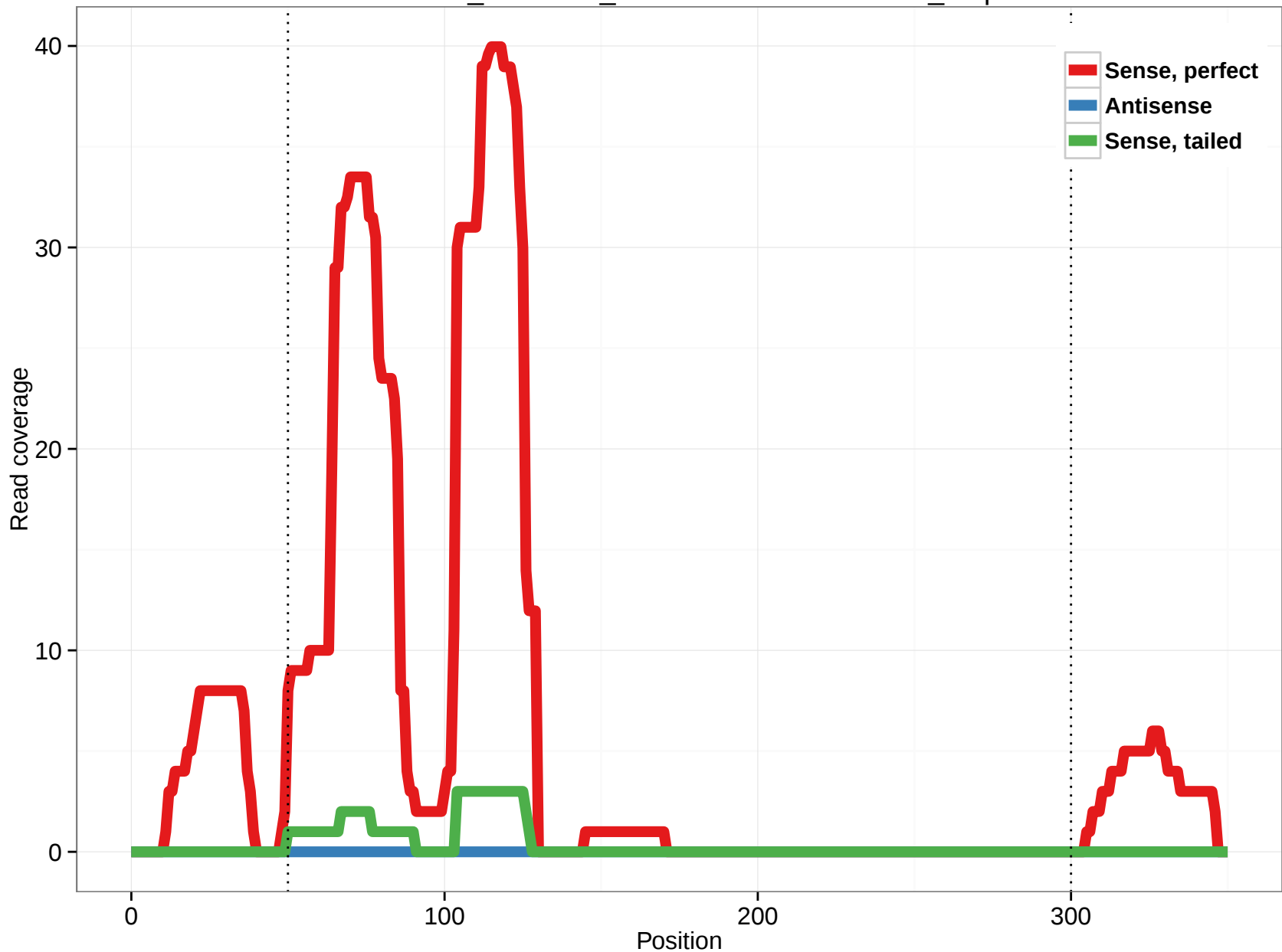
ornAna1_ensGene_ENSOANT00000019314_2.3p
