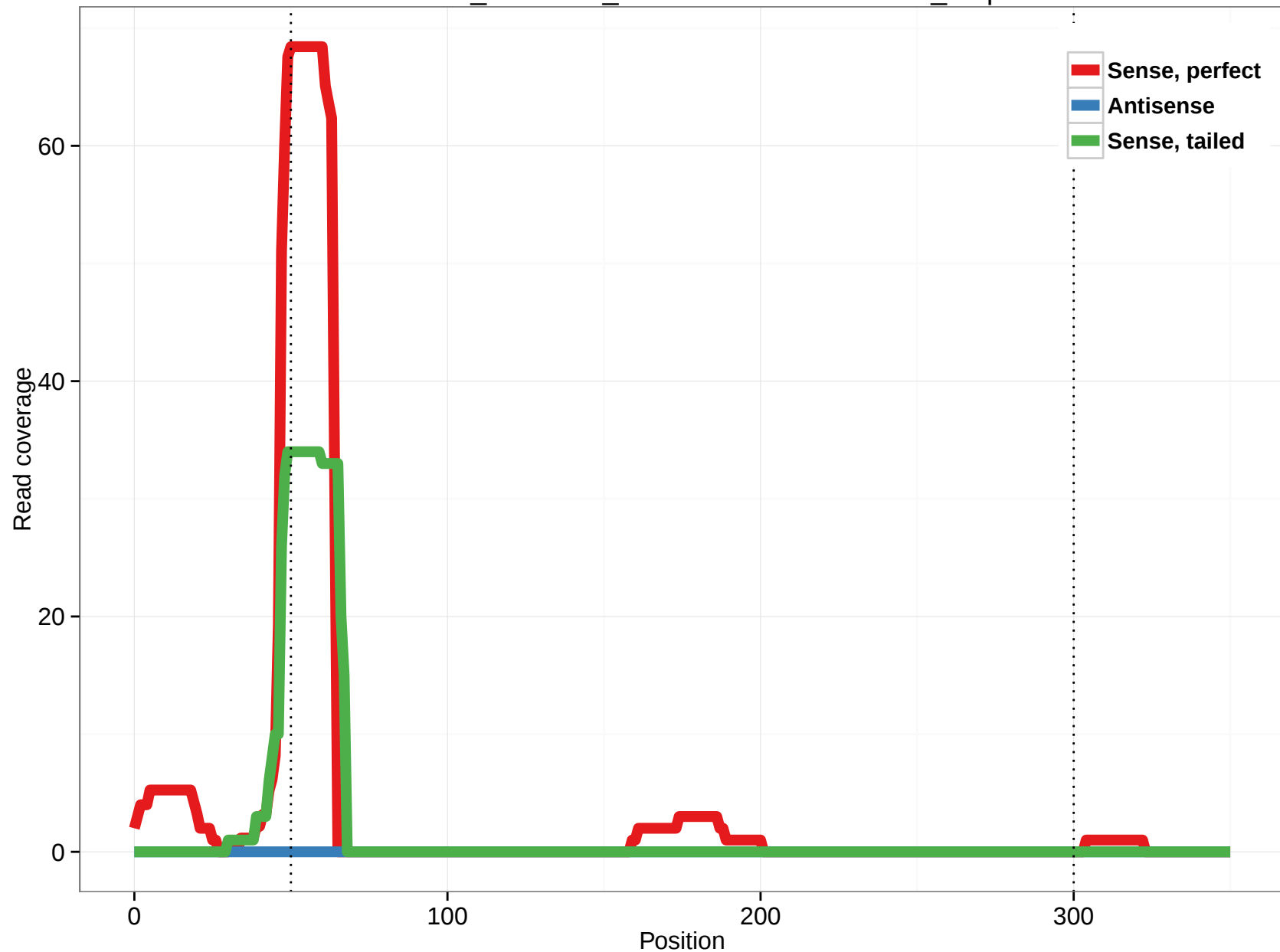
ornAna1_ensGene_ENSOANT00000019182_1.5p
