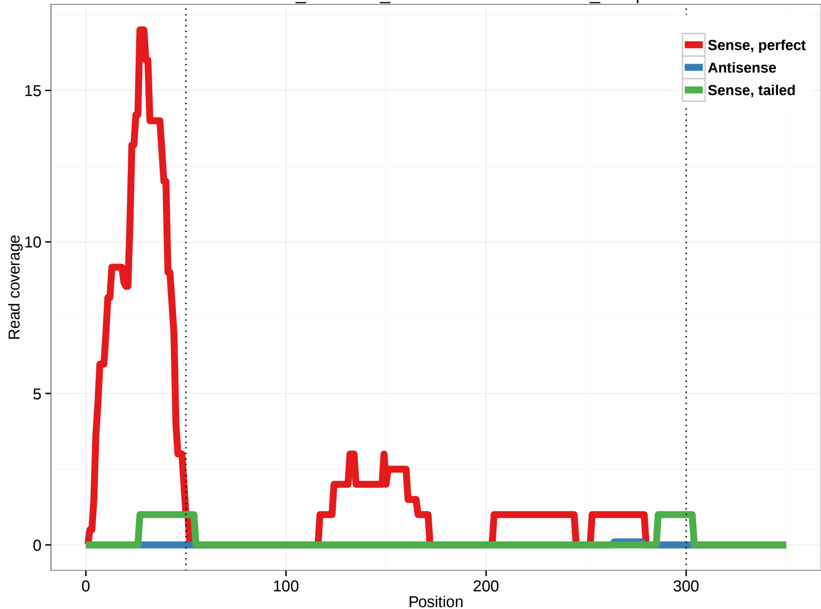
ornAna1_ensGene_ENSOANT00000019181_10.5p
