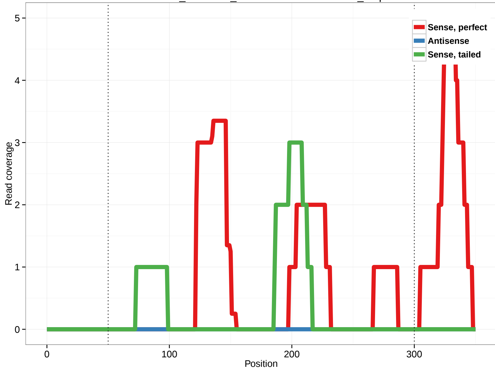
ornAna1_ensGene_ENSOANT00000019167_4.3p
